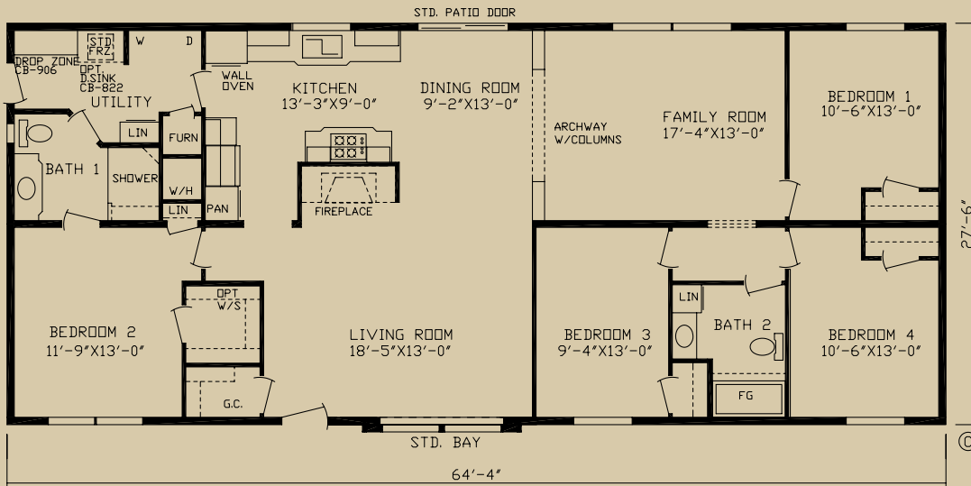
The Waterbury Model # 161000 1760 Sq. Ft.
